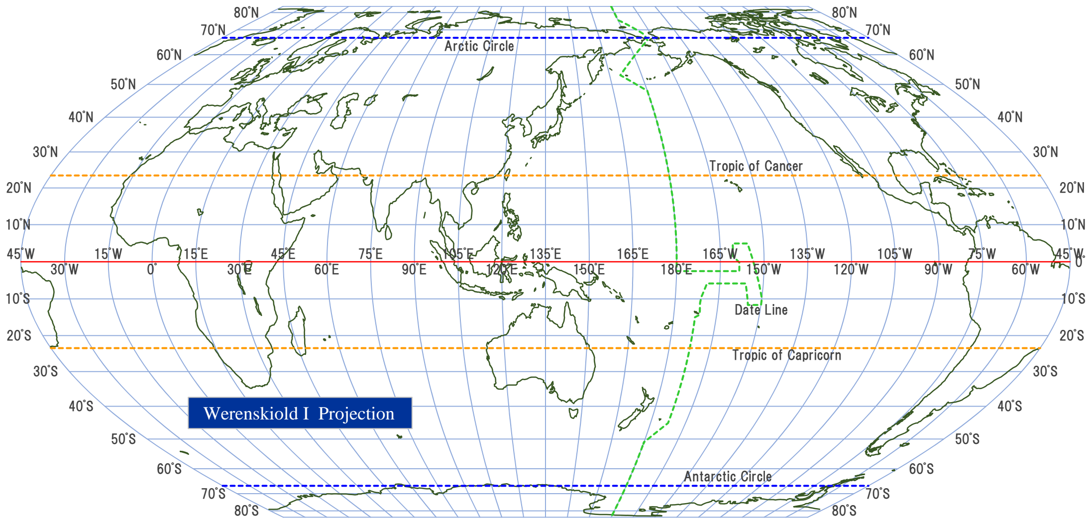
[ 図 6-2-1-32 ] Werenskiöld I Projection
