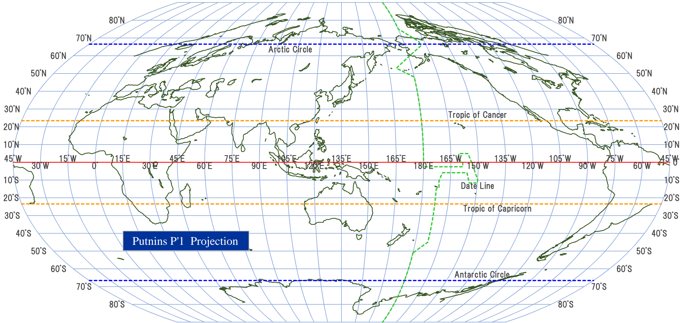
[ 図 6-2-1-28 ] Putnins P'1 Projection
