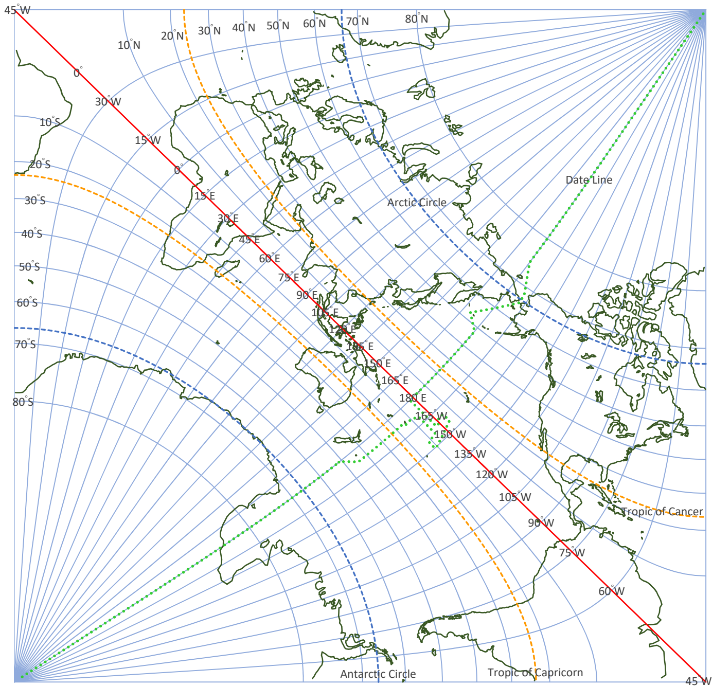
[図 6-7-2-7] Adams World in a Square II 図法 ( Adams World in a Square II Projection )
