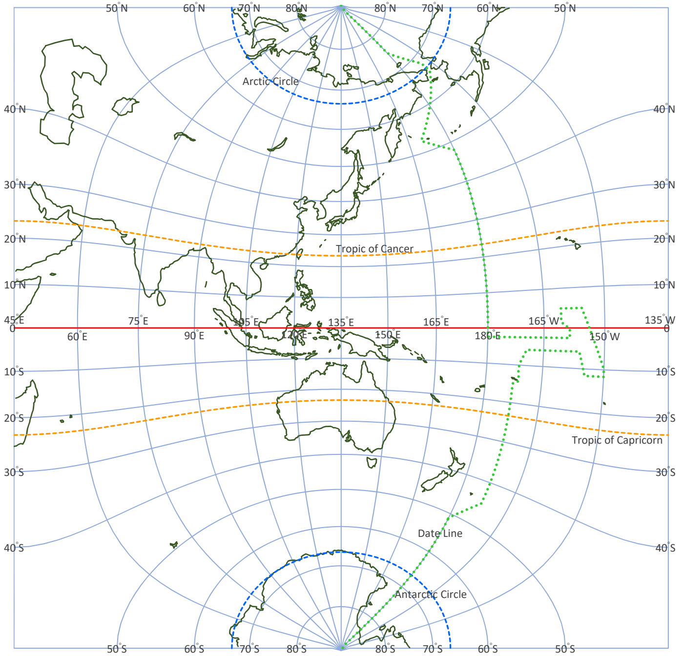
[図 6-7-2-1] Guyou 図法 (Guyou Projection)
