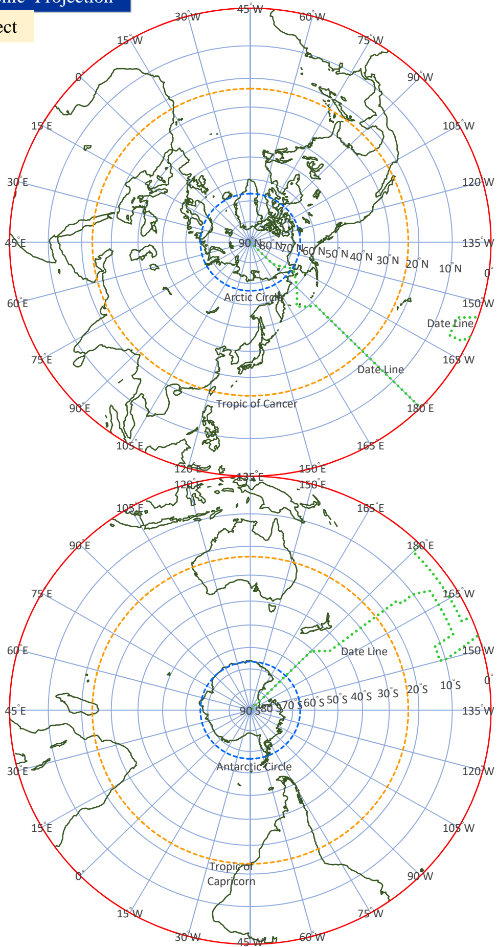
[圖 6-5-1-2-1] 平射圖法 - 極面、半球縱列 ( Stereographic Projection,Polar Aspect )
