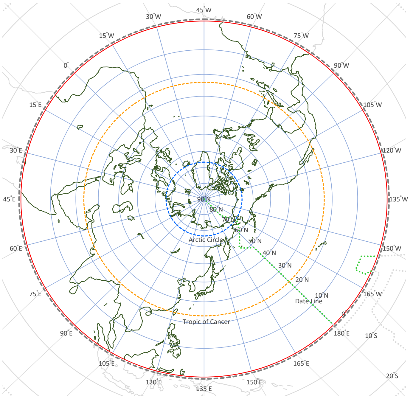
[図 6-5-1-2-1] 平射図法 - 極面 ( Stereographic Projection,Polar Aspect )
