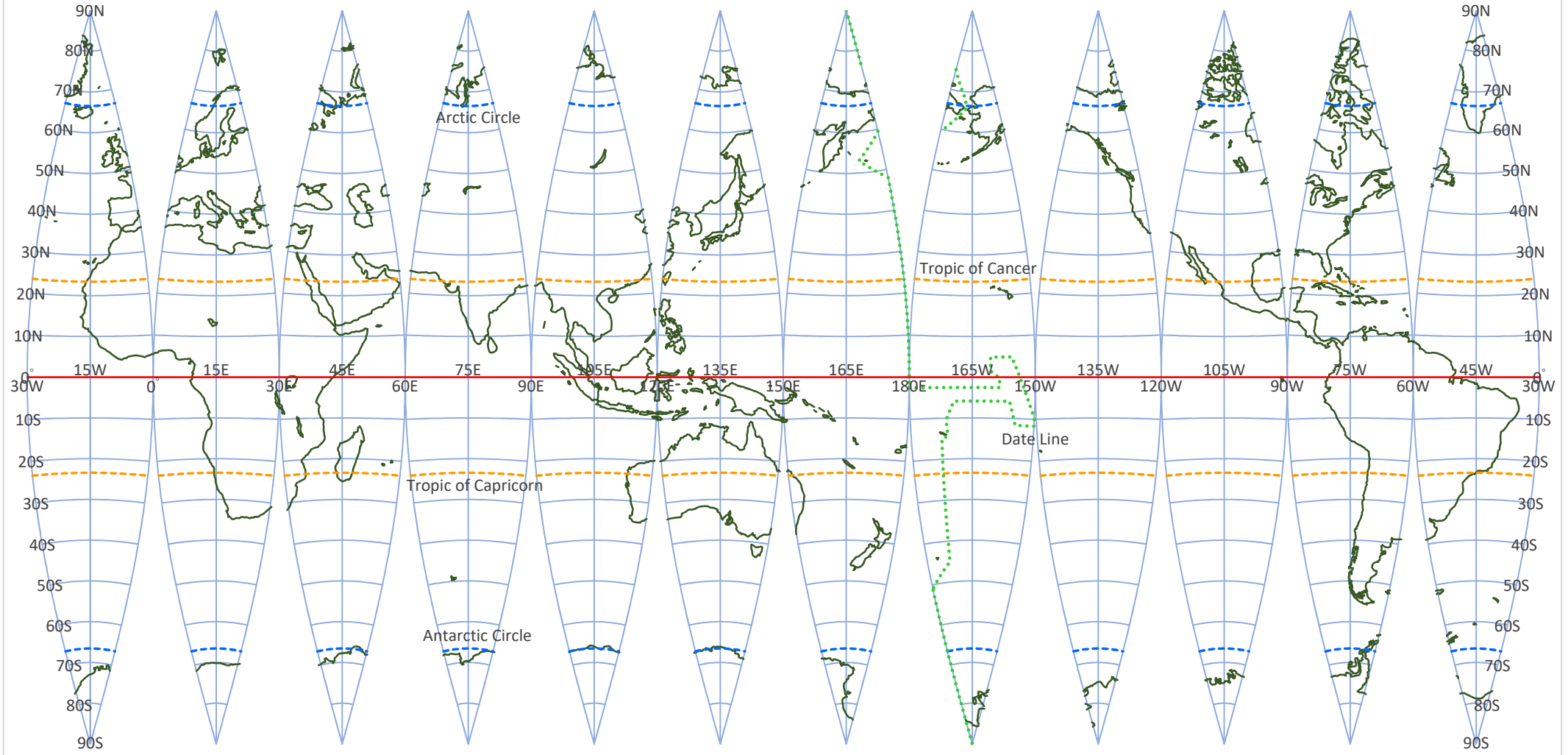
[图 6-3-8] 断裂多圆锥图法 (舟底型多圆锥图法・Interrupted Normal Polyconic Projection)
